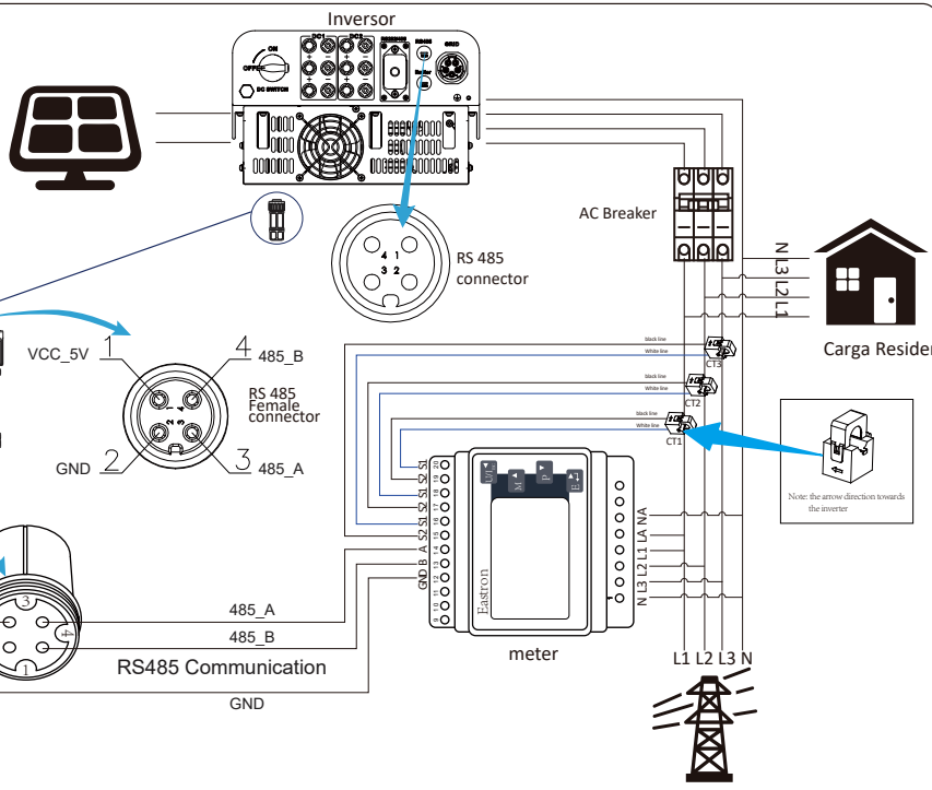
Eastron SDM630MCT Figura 7.12 Medidor Eastron
